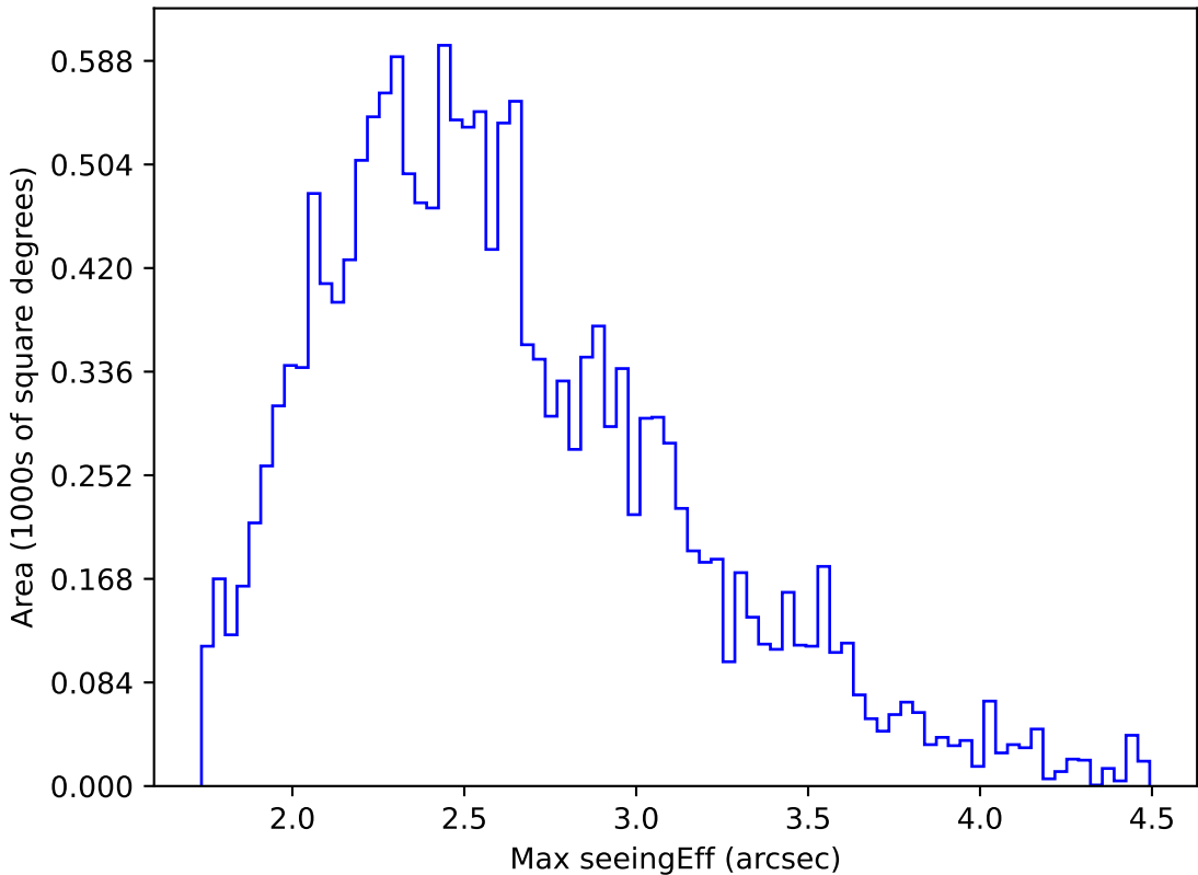
too_elab_r128_d3_gz_v3.4_10yrs WFD g band: Max seeingEff
