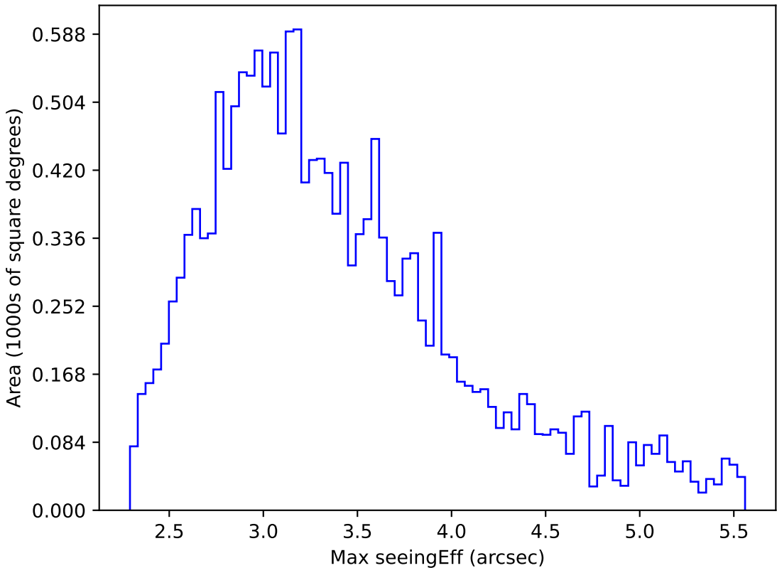
too_elab_r128_d3_gz_v3.4_10yrs WFD all bands: Max seeingEff
