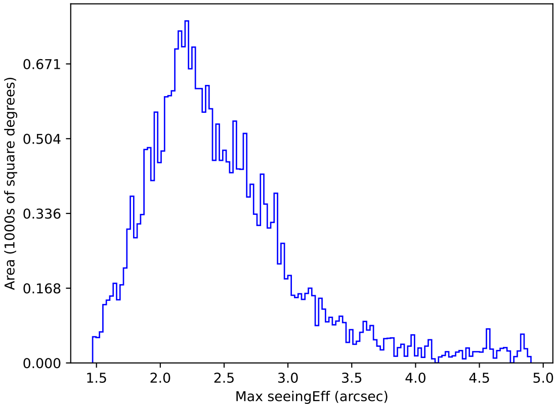
too_elab_r128_d3_gz_v3.4_10yrs All sky z band: Max seeingEff
