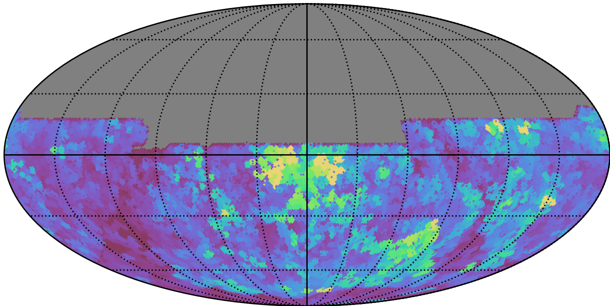
too_elab_r128_d3_gz_v3.4_10yrs All sky y band: Max seeingEff
