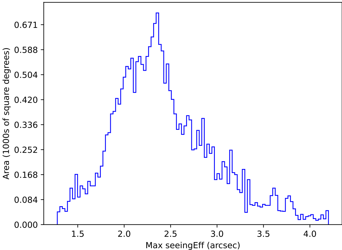
too_elab_r128_d3_gz_v3.4_10yrs All sky u band: Max seeingEff
