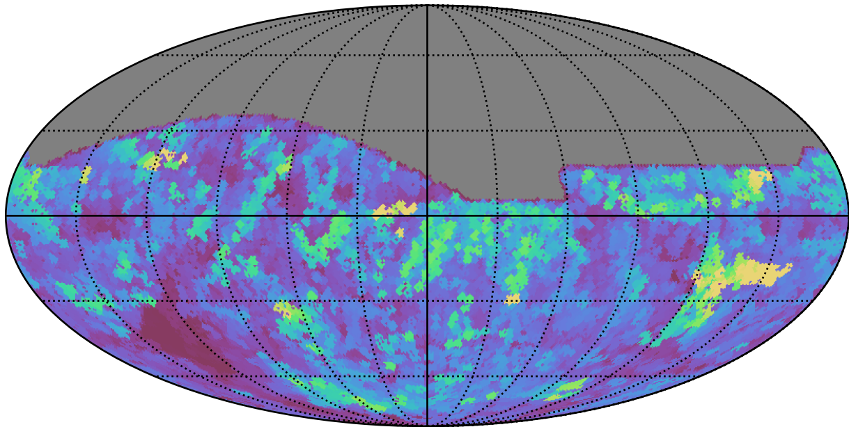
too_elab_r128_d3_gz_v3.4_10yrs All sky r band: Max seeingEff
