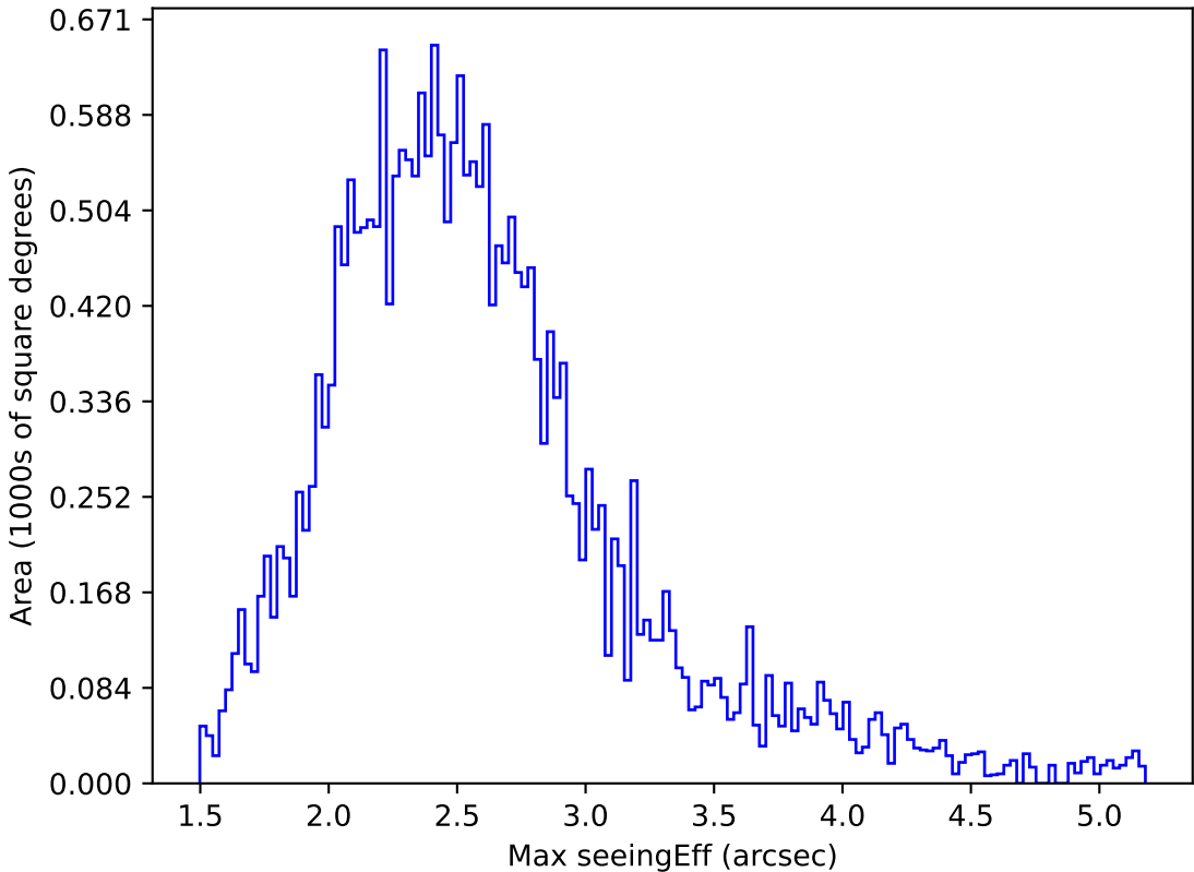
too_elab_r128_d3_gz_v3.4_10yrs All sky i band: Max seeingEff
