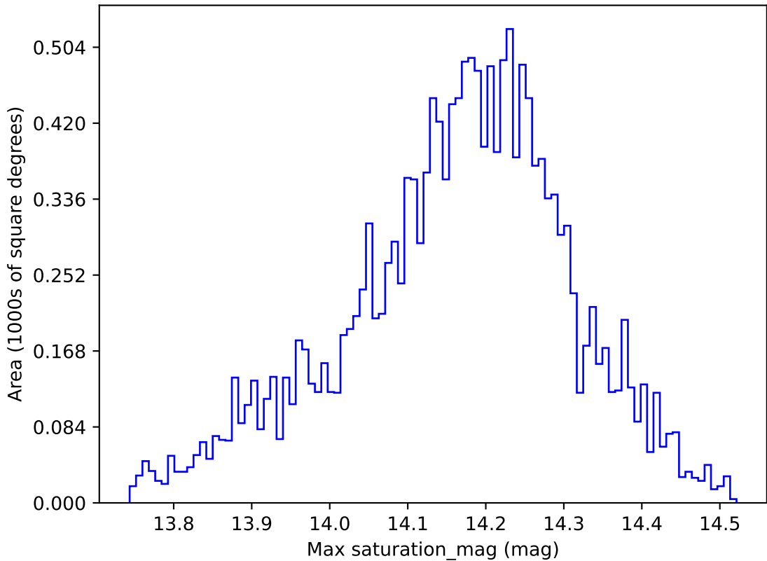
too_elab_r128_d3_gz_v3.4_10yrs WFD y band: Max saturation_mag
