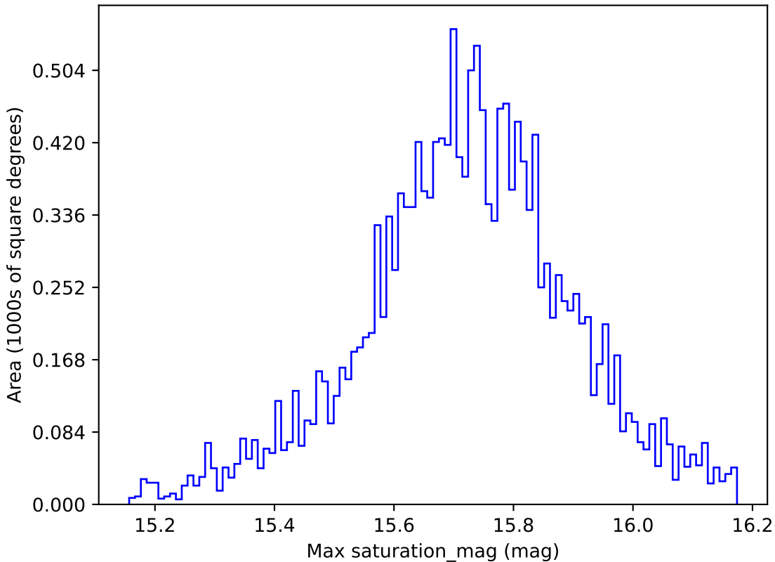
too_elab_r128_d3_gz_v3.4_10yrs WFD g band: Max saturation_mag
