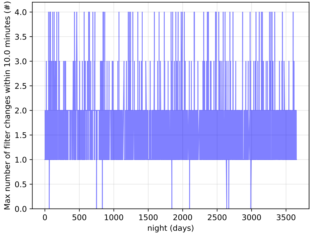
too_elab_r128_d3_gz_v3.4_10yrs Per Night: Max number of filter changes within 10.0 minutes
