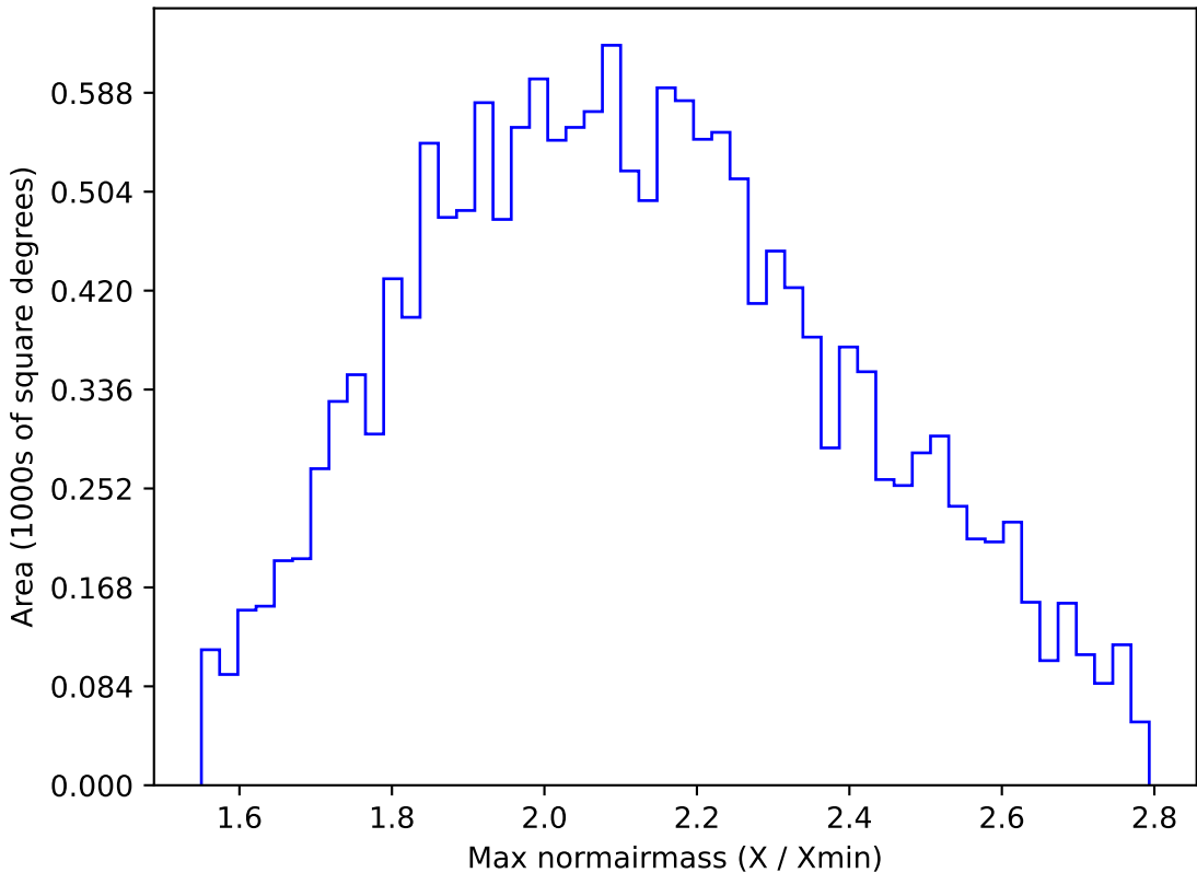
too_elab_r128_d3_gz_v3.4_10yrs WFD y band: Max normairmass
