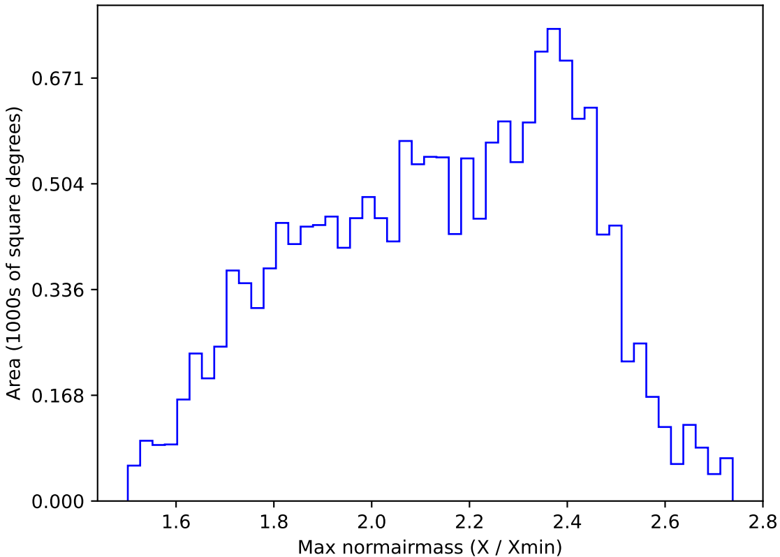
too_elab_r128_d3_gz_v3.4_10yrs WFD r band: Max normairmass
