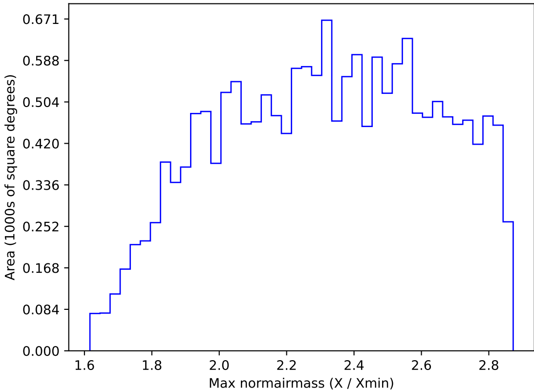
too_elab_r128_d3_gz_v3.4_10yrs WFD i band: Max normairmass
