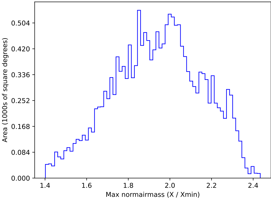
too_elab_r128_d3_gz_v3.4_10yrs WFD g band: Max normairmass
