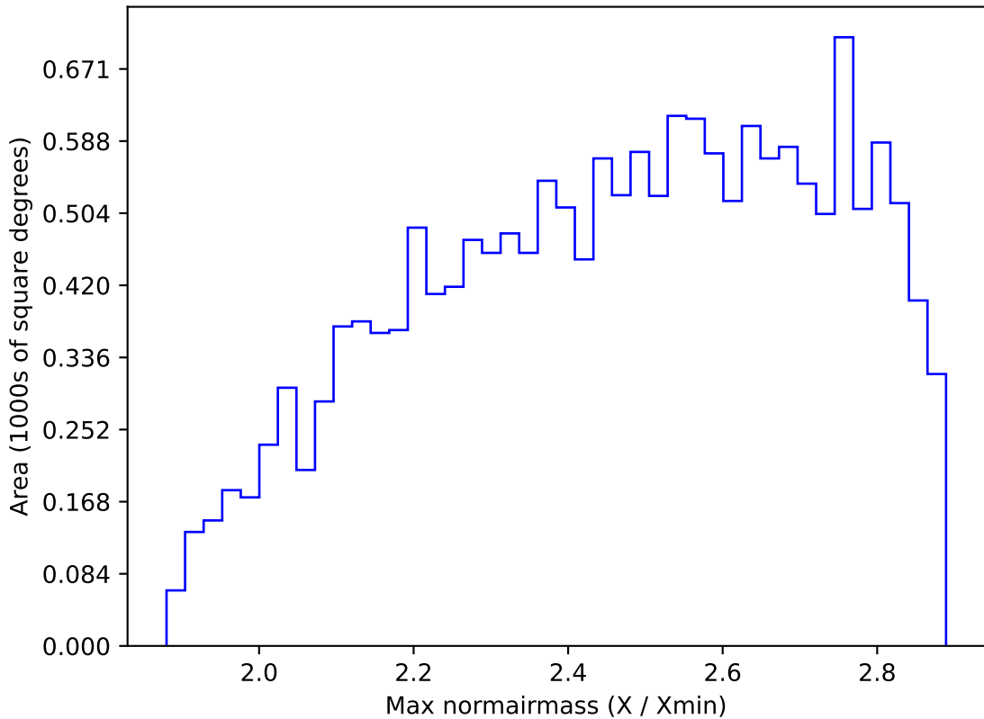
too_elab_r128_d3_gz_v3.4_10yrs WFD all bands: Max normairmass
