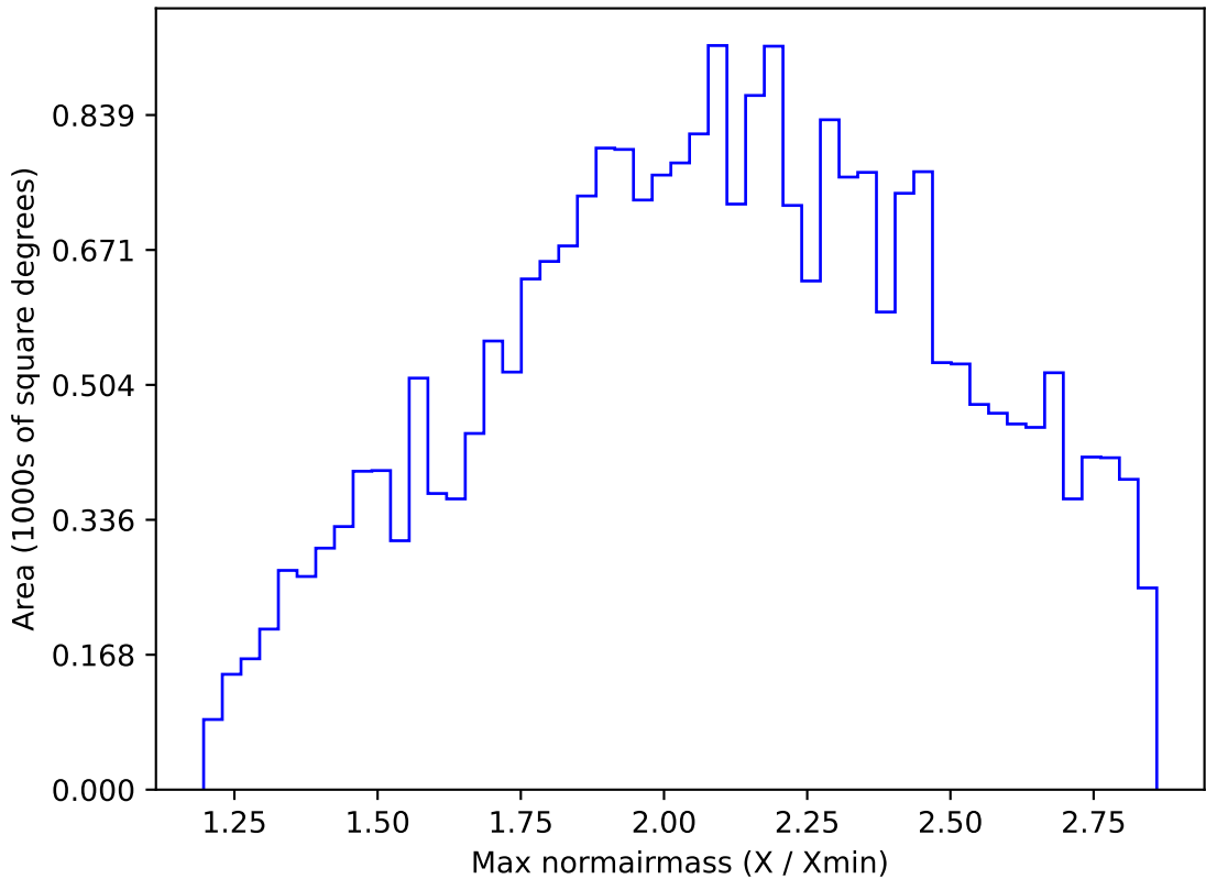
too_elab_r128_d3_gz_v3.4_10yrs All sky z band: Max normairmass
