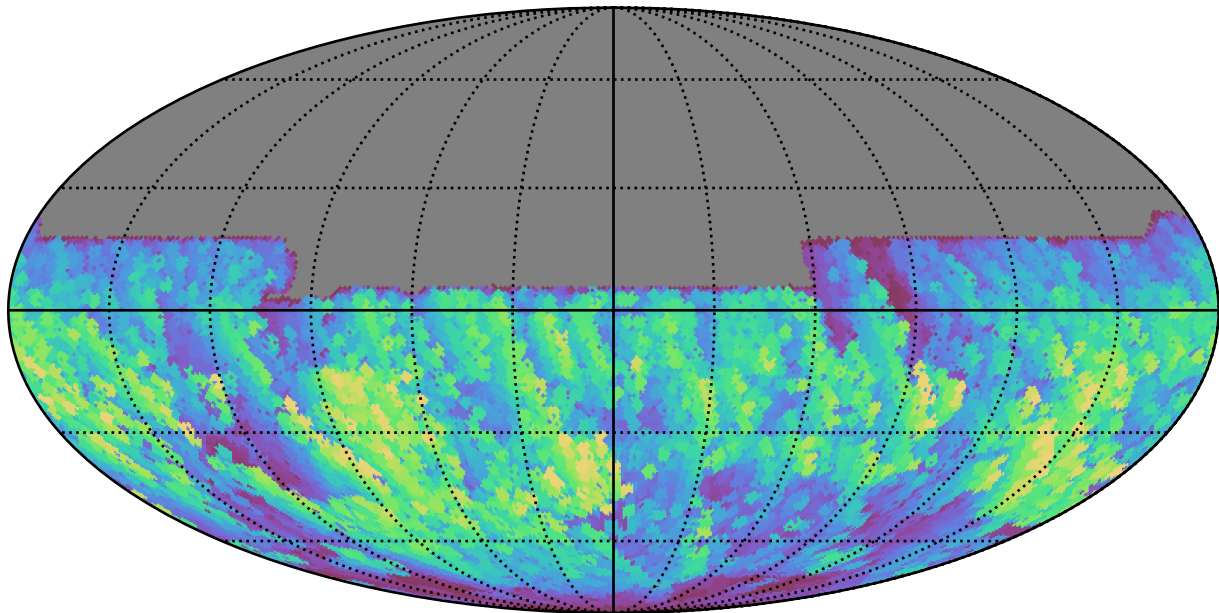
too_elab_r128_d3_gz_v3.4_10yrs All sky y band: Max normairmass
