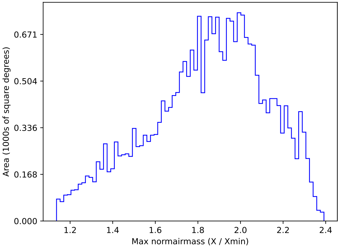
too_elab_r128_d3_gz_v3.4_10yrs All sky g band: Max normairmass
