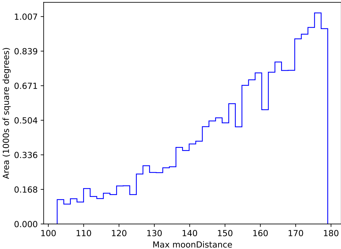
too_elab_r128_d3_gz_v3.4_10yrs WFD z band: Max moonDistance
