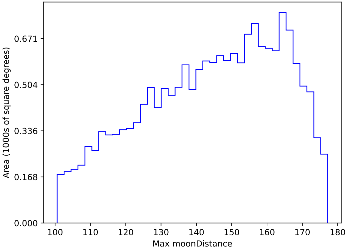
too_elab_r128_d3_gz_v3.4_10yrs WFD y band: Max moonDistance
