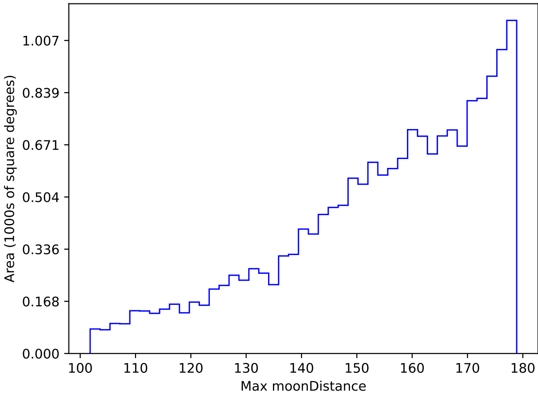
too_elab_r128_d3_gz_v3.4_10yrs WFD u band: Max moonDistance
