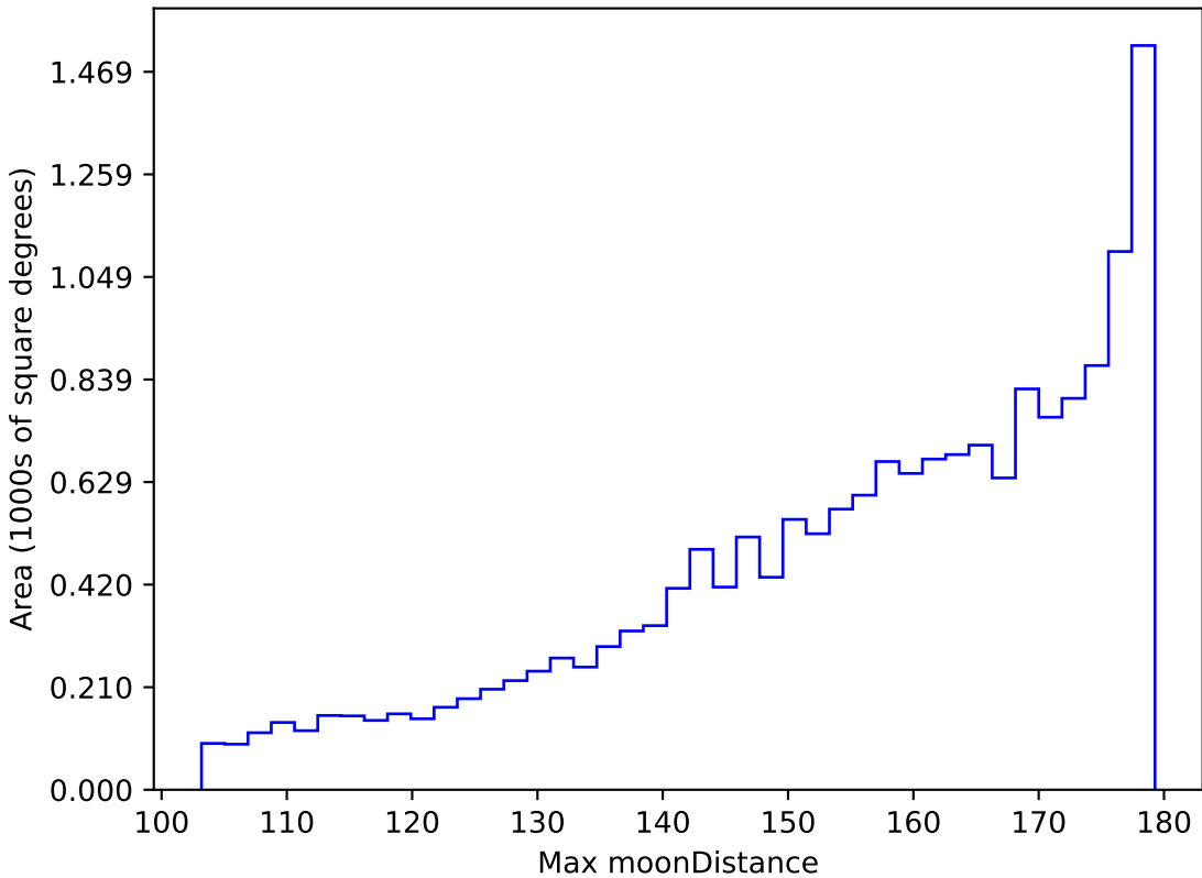
too_elab_r128_d3_gz_v3.4_10yrs WFD r band: Max moonDistance
