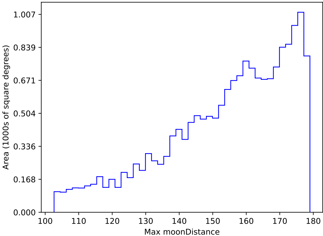
too_elab_r128_d3_gz_v3.4_10yrs WFD g band: Max moonDistance
