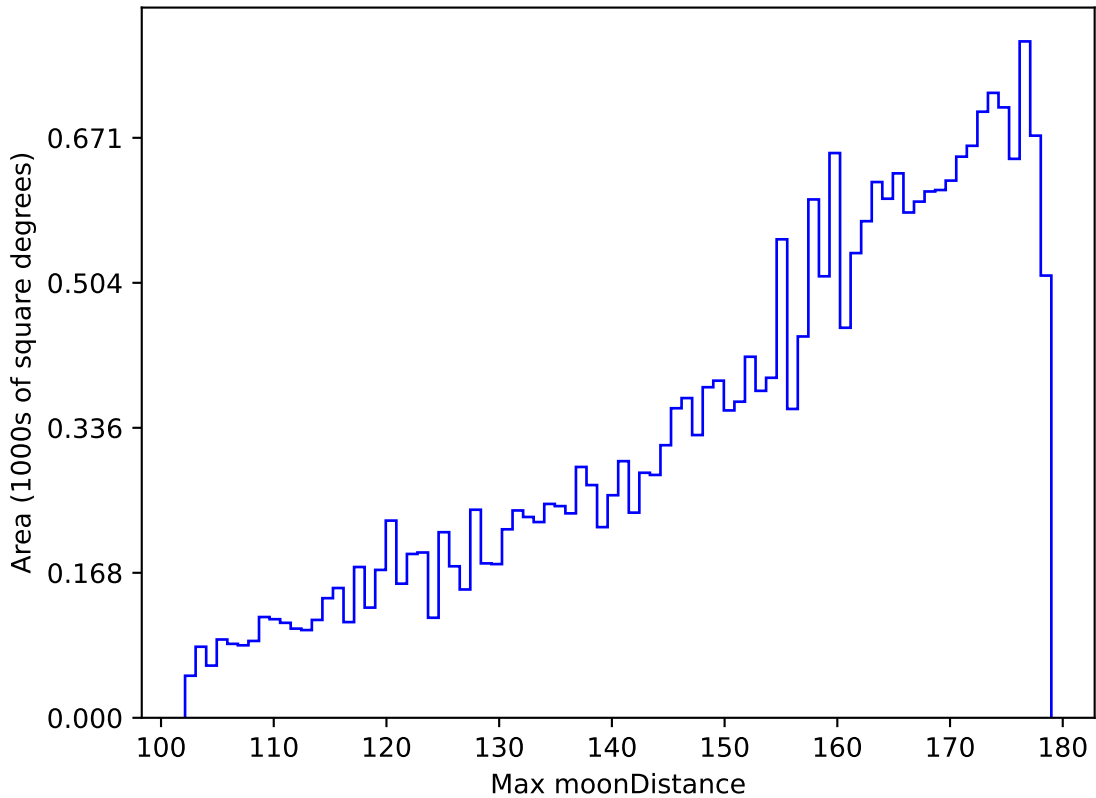
too_elab_r128_d3_gz_v3.4_10yrs All sky z band: Max moonDistance
