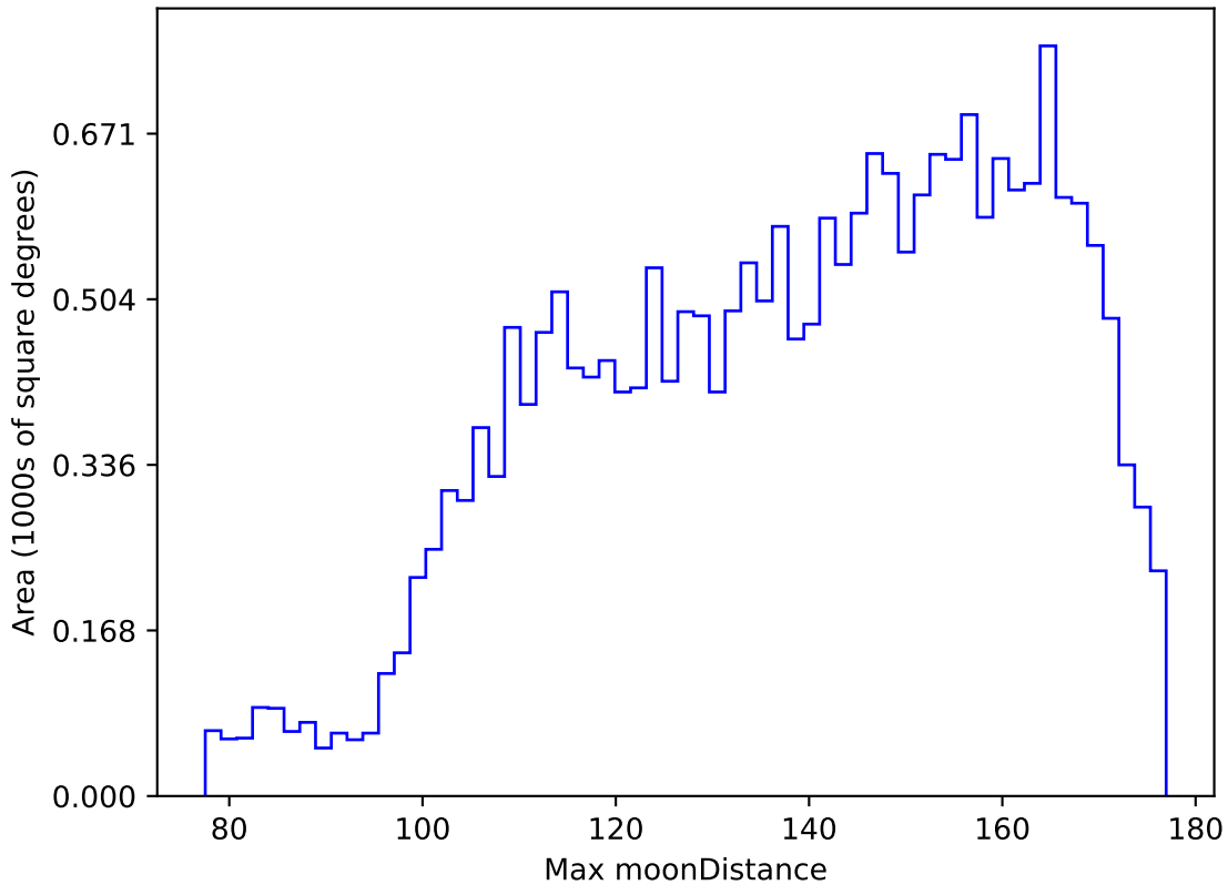
too_elab_r128_d3_gz_v3.4_10yrs All sky y band: Max moonDistance
