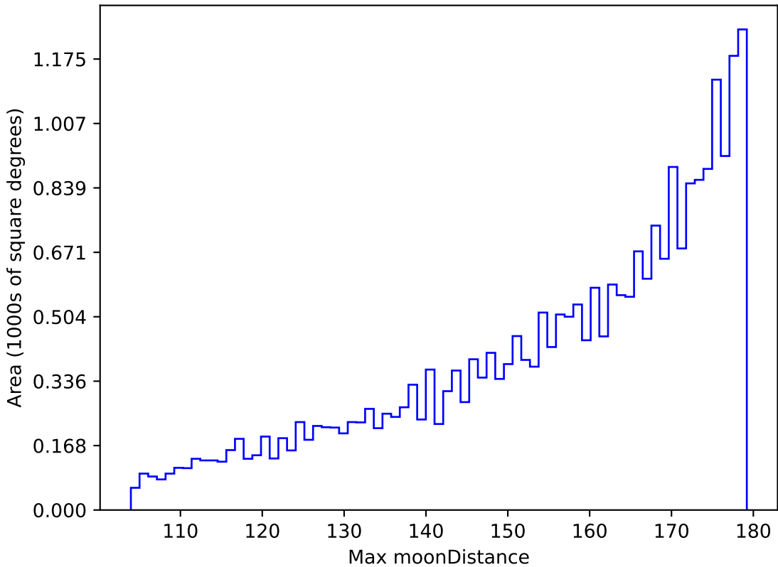
too_elab_r128_d3_gz_v3.4_10yrs All sky r band: Max moonDistance
