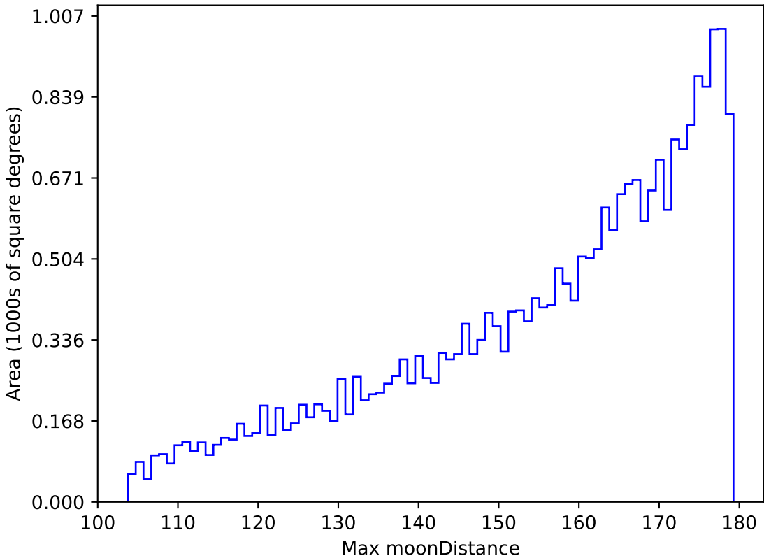
too_elab_r128_d3_gz_v3.4_10yrs All sky i band: Max moonDistance
