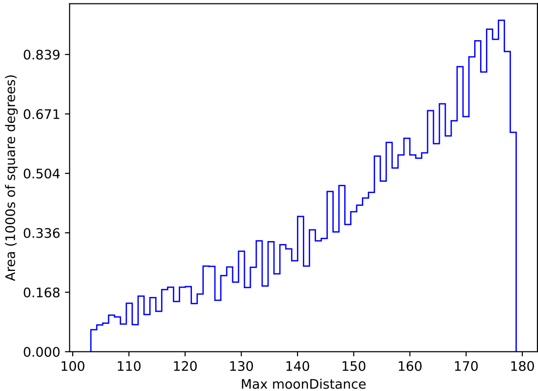
too_elab_r128_d3_gz_v3.4_10yrs All sky g band: Max moonDistance
