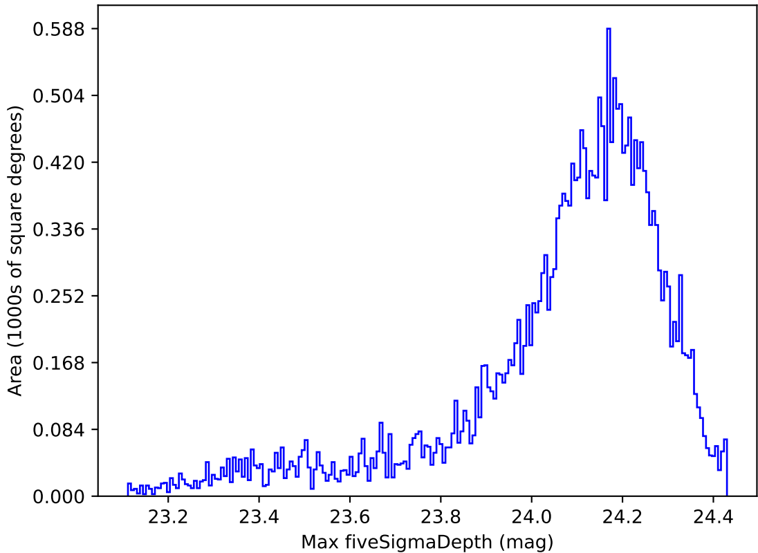
too_elab_r128_d3_gz_v3.4_10yrs Yr 1 i band: Max fiveSigmaDepth
