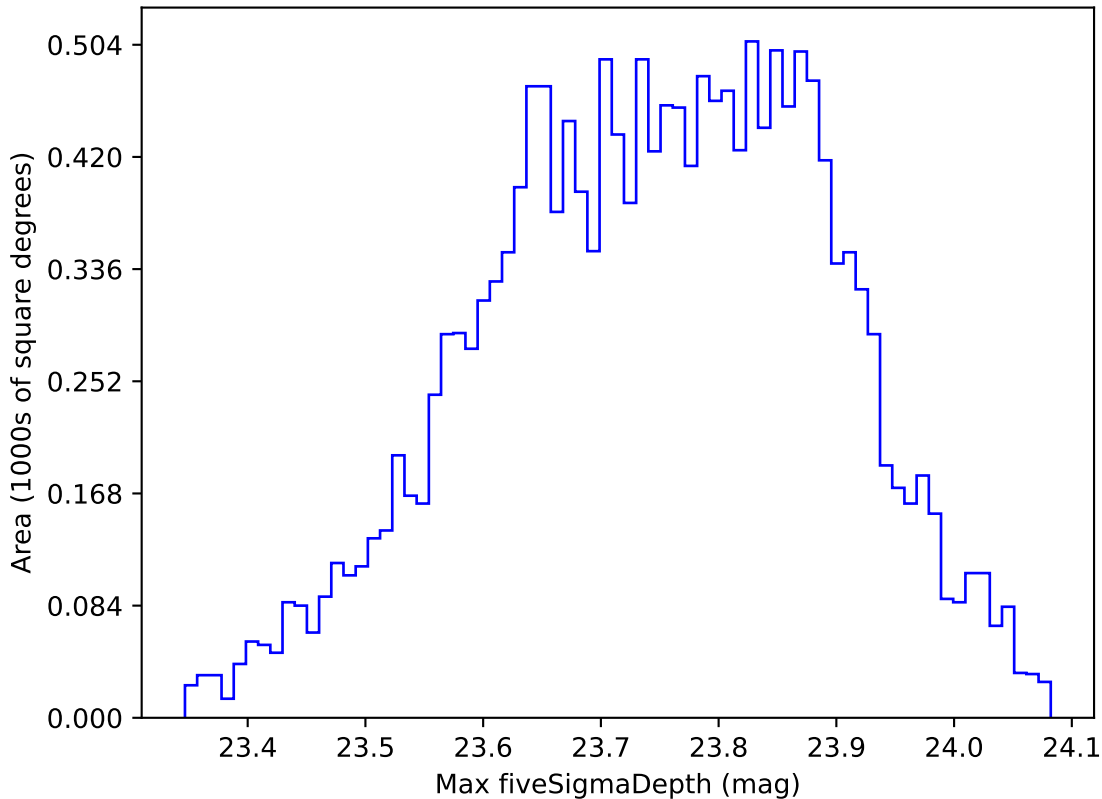
too_elab_r128_d3_gz_v3.4_10yrs WFD u band: Max fiveSigmaDepth
