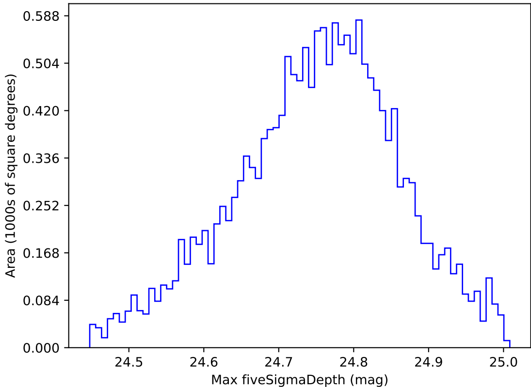
too_elab_r128_d3_gz_v3.4_10yrs WFD r band: Max fiveSigmaDepth
