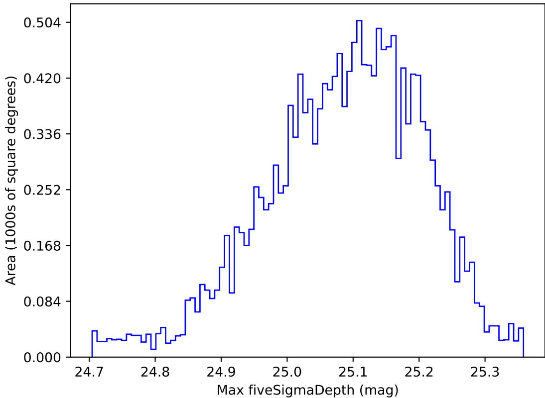
too_elab_r128_d3_gz_v3.4_10yrs WFD g band: Max fiveSigmaDepth
