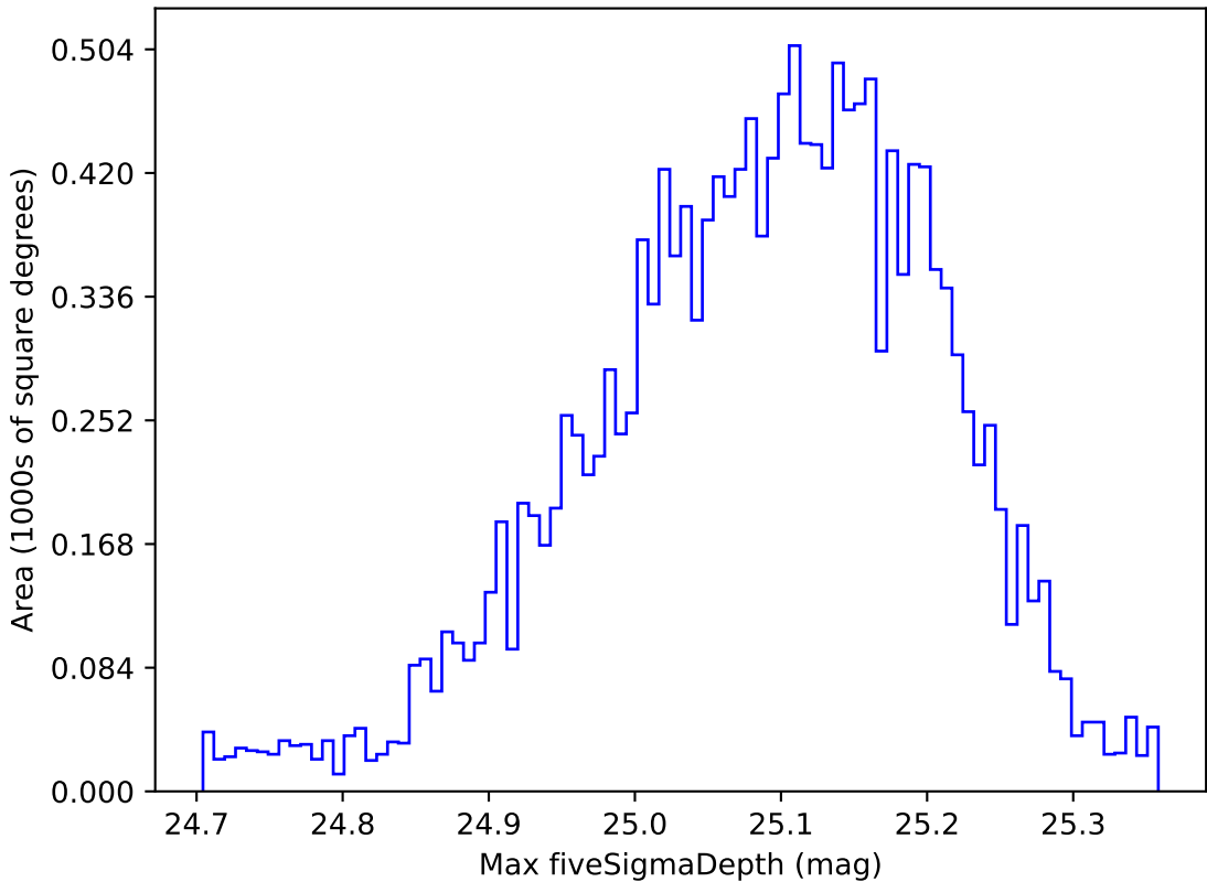
too_elab_r128_d3_gz_v3.4_10yrs WFD all bands: Max fiveSigmaDepth
