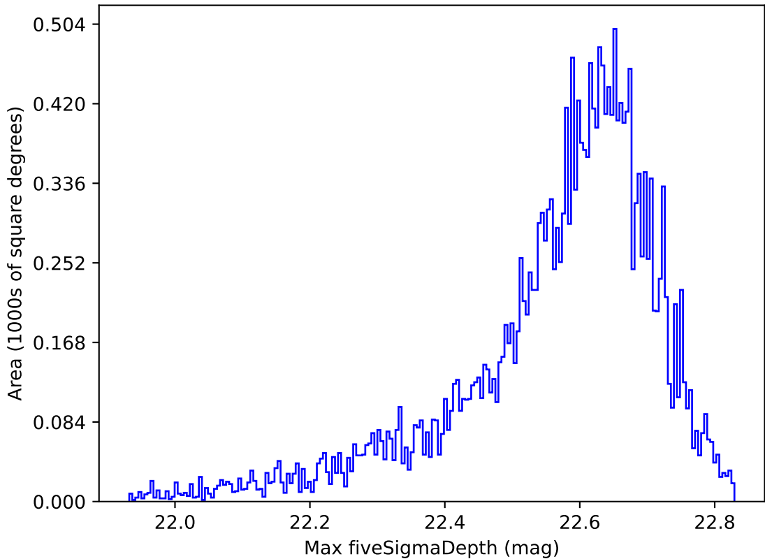
too_elab_r128_d3_gz_v3.4_10yrs All sky y band: Max fiveSigmaDepth
