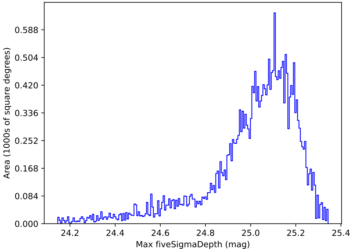
too_elab_r128_d3_gz_v3.4_10yrs All sky g band: Max fiveSigmaDepth
