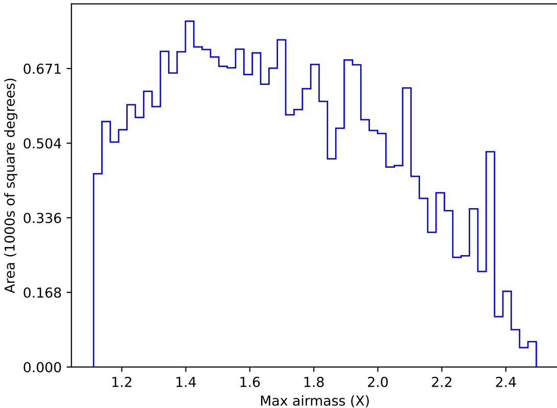
too_elab_r128_d3_gz_v3.4_10yrs Yr 1 g band: Max airmass
