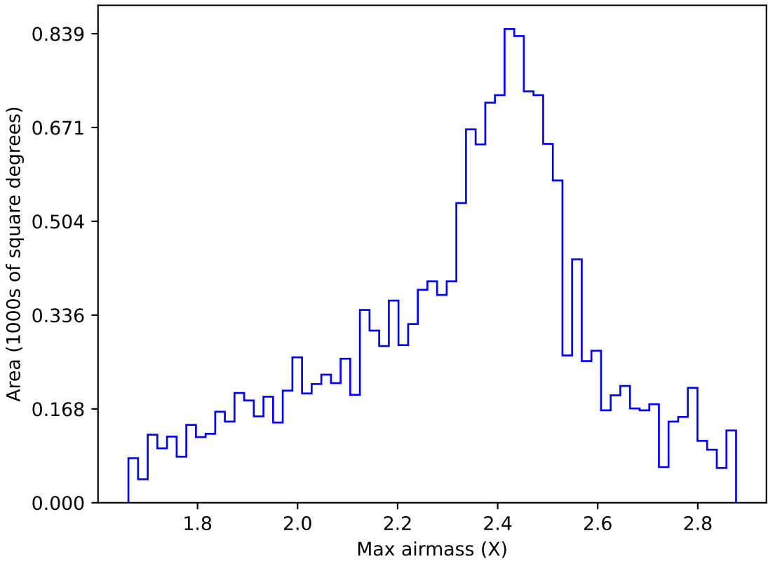
too_elab_r128_d3_gz_v3.4_10yrs WFD r band: Max airmass
