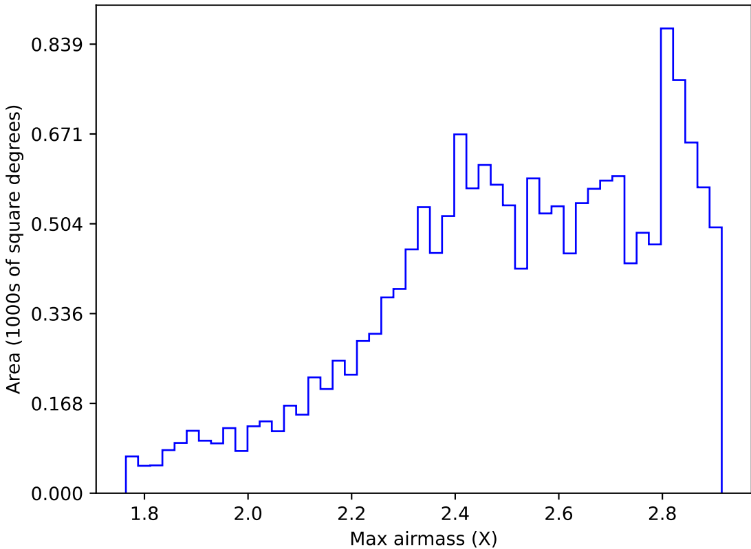
too_elab_r128_d3_gz_v3.4_10yrs WFD i band: Max airmass
