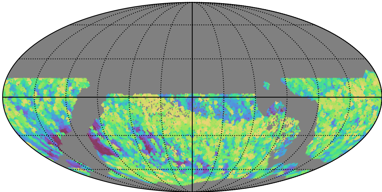
too_elab_r128_d3_gz_v3.4_10yrs WFD all bands: Max airmass
