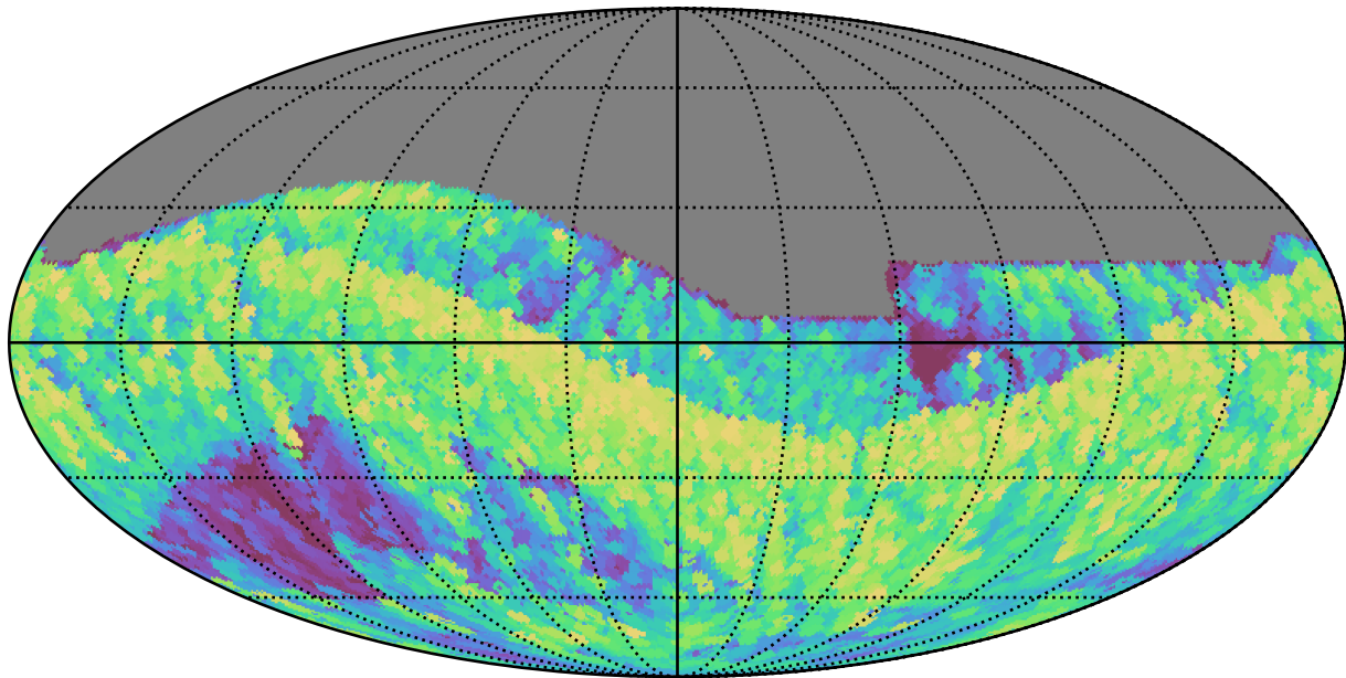
too_elab_r128_d3_gz_v3.4_10yrs All sky i band: Max airmass
