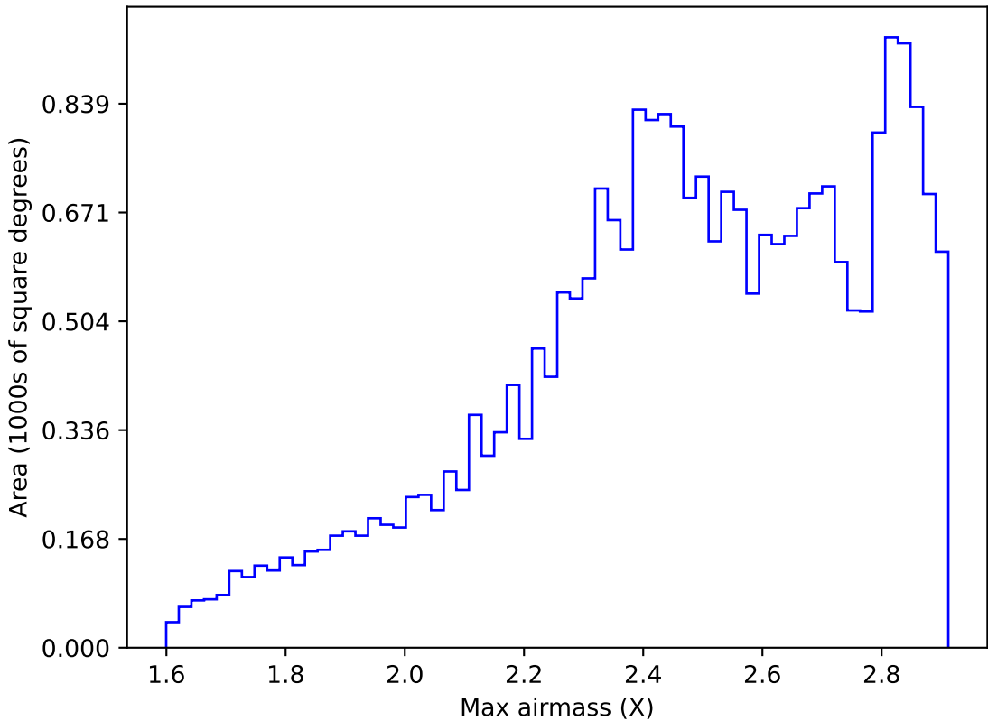
too_elab_r128_d3_gz_v3.4_10yrs All sky i band: Max airmass
