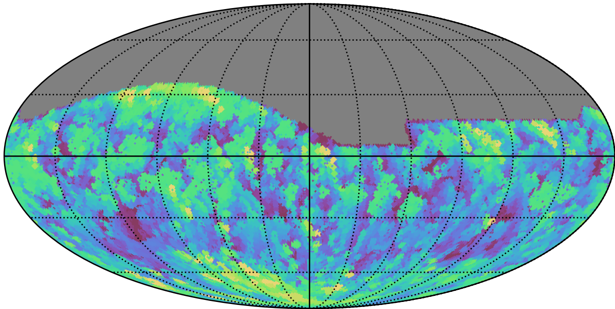
too_elab_r128_d3_gz_v3.4_10yrs All sky g band: Max airmass
