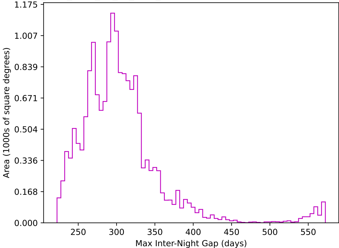
too_elab_r128_d3_gz_v3.4_10yrs WFD z band: Max Inter-Night Gap
