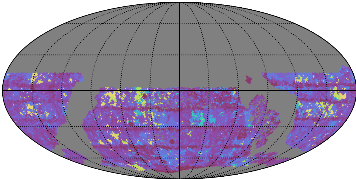
too_elab_r128_d3_gz_v3.4_10yrs WFD y band: Max Inter-Night Gap
