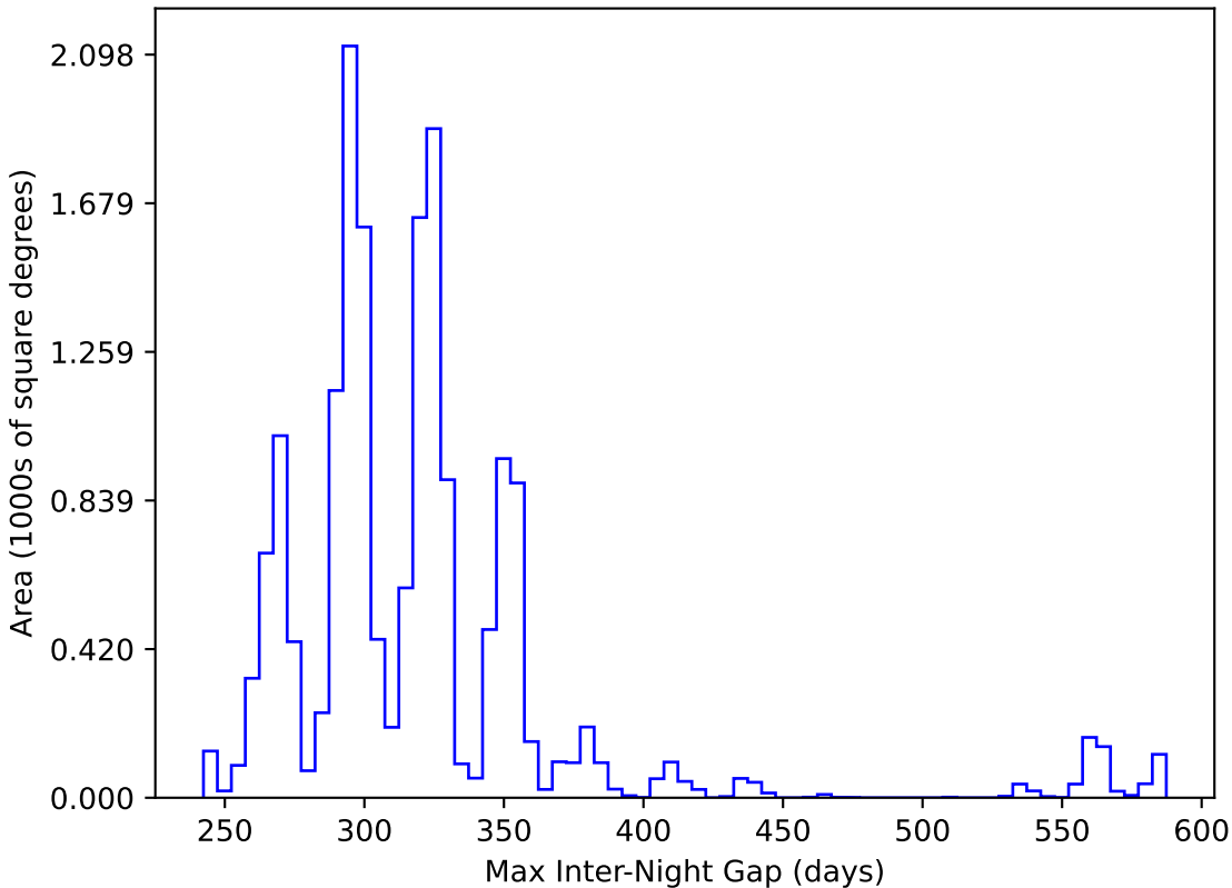
too_elab_r128_d3_gz_v3.4_10yrs WFD y band: Max Inter-Night Gap
