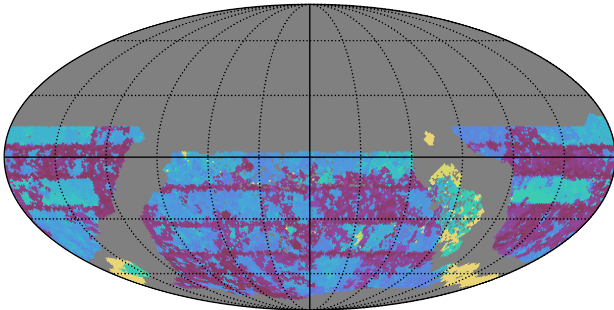
too_elab_r128_d3_gz_v3.4_10yrs WFD u band: Max Inter-Night Gap
