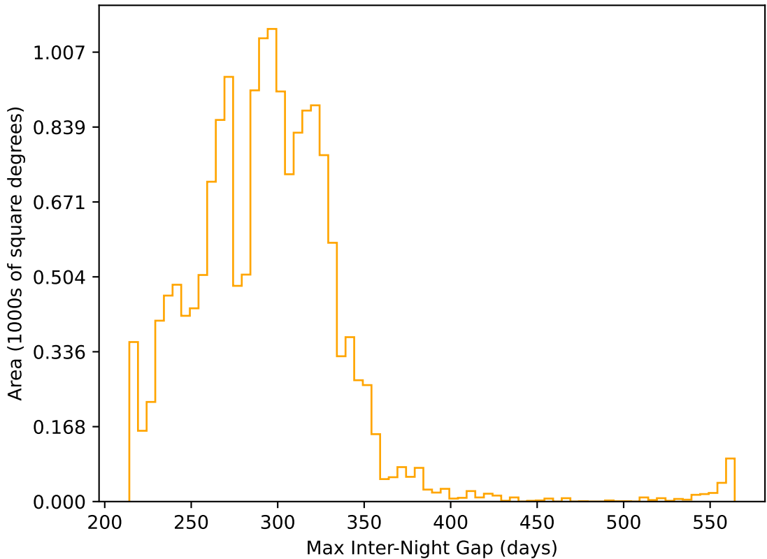
too_elab_r128_d3_gz_v3.4_10yrs WFD r band: Max Inter-Night Gap
