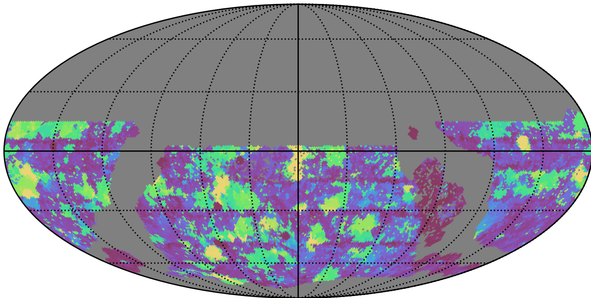
too_elab_r128_d3_gz_v3.4_10yrs WFD g band: Max Inter-Night Gap
