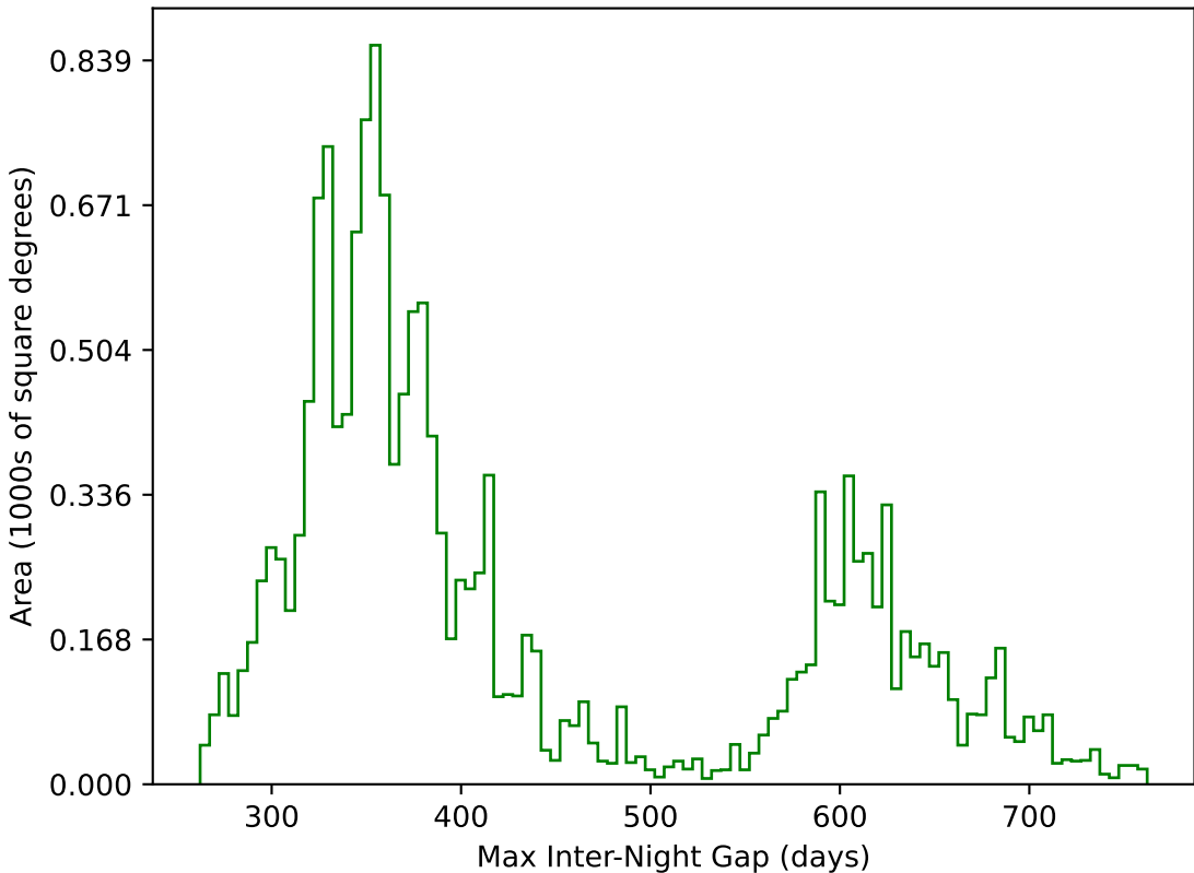
too_elab_r128_d3_gz_v3.4_10yrs WFD g band: Max Inter-Night Gap
