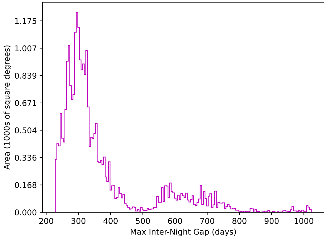
too_elab_r128_d3_gz_v3.4_10yrs All sky z band: Max Inter-Night Gap
